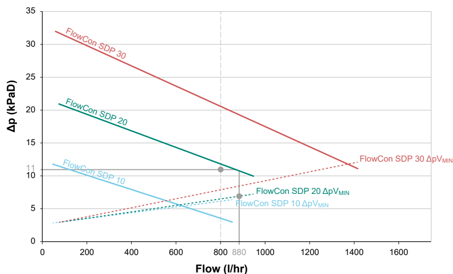
Controlled \Delta p_C circuit and \Delta p_{V_{MIN}}
